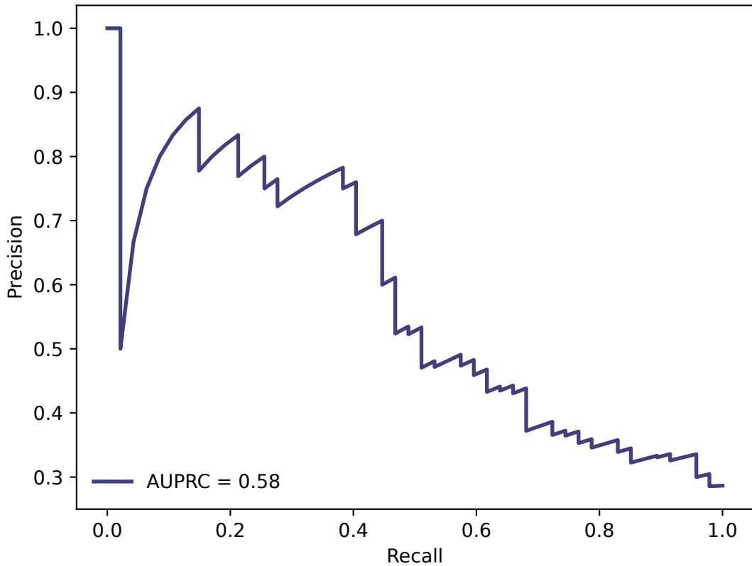
RF Precision-Recall Curve
